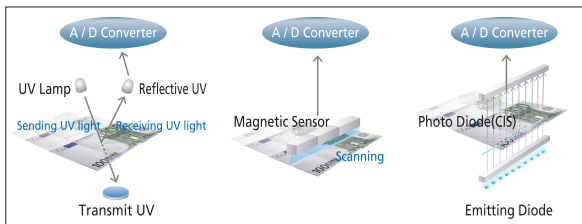
<Ultraviolet Sensor> <Magnetic Sensor> <Infrared Sensor>
